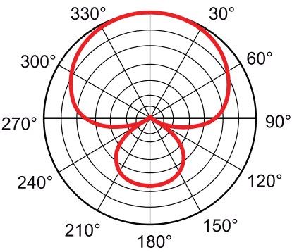
Supercardioid Polar Pattern
