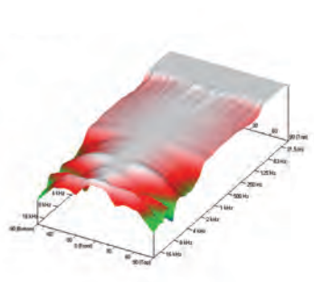
Directivity of a single speaker
